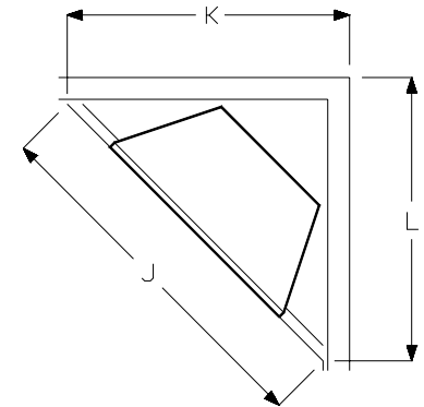
Rough-in corner framing
