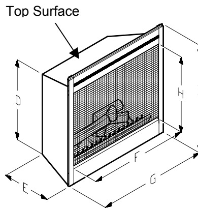
Firebox dimensions
